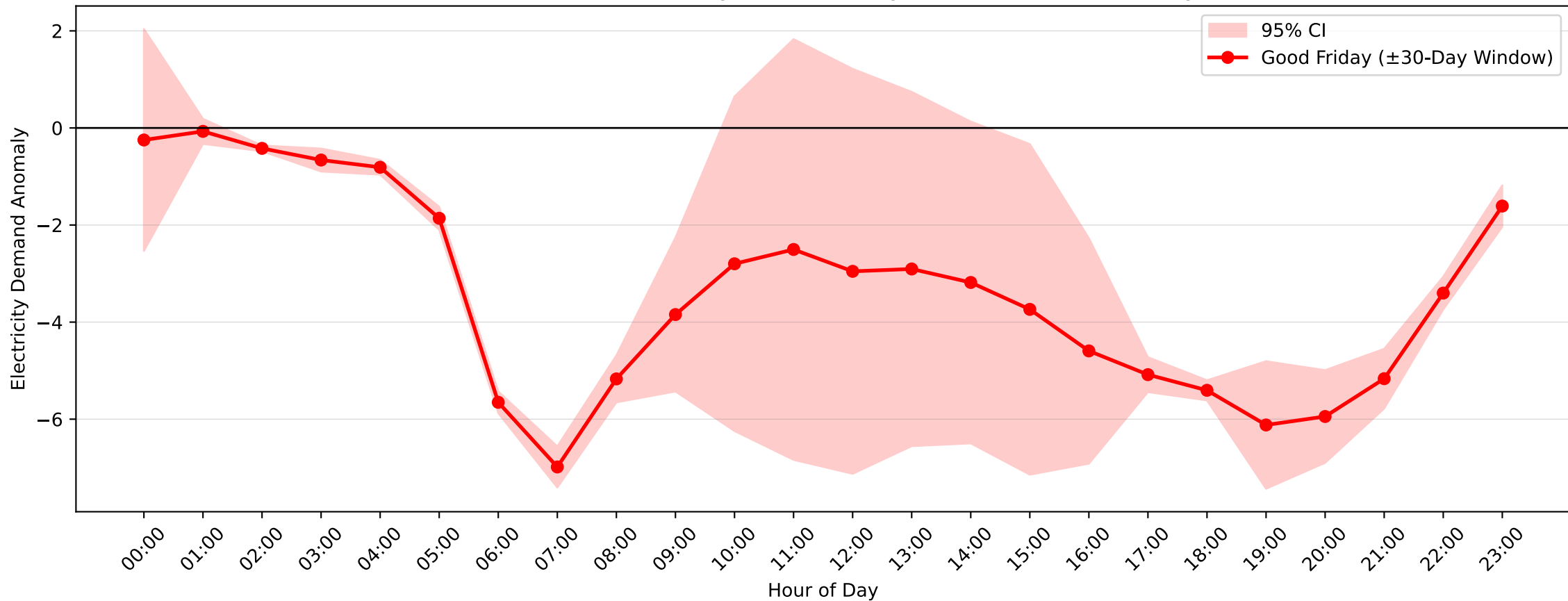
Pennant Hills Demand Anomaly: Good Friday (2014-2015, \pm 30 -Day Window)
