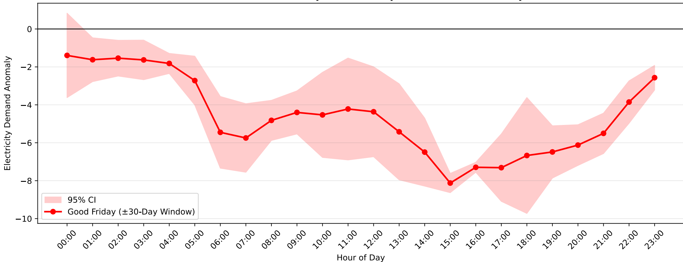
Pennant Hills Demand Anomaly: Good Friday (2016–2017, \pm 30 -Day Window)
